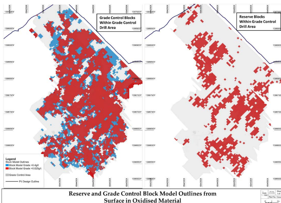
Figure Thirty Three | Near Surface Grade Control to Reserve Comparison
